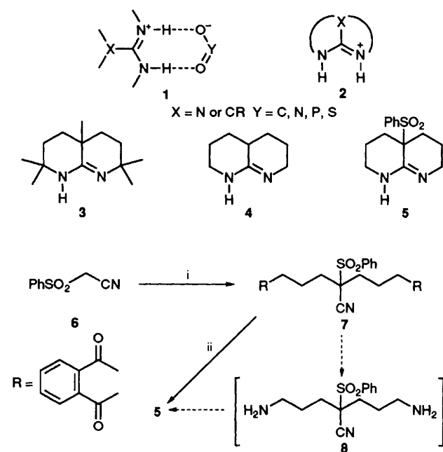
Scheme 1 Reagents and conditions: i, N -(3-bromopropyl)phthalimide (2.2 equiv.), DBU (2.2 equiv.), DMF, 80 °C, 40 min; ii, NaBH 4 , Pr i OH, H 2 O, room temp., 24 h, followed by addition of AcOH, 80 °C, 3 h
