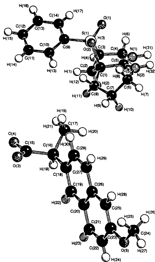
Fig. 2 X-Ray crystal structure of 5H^+ naxproxenate
