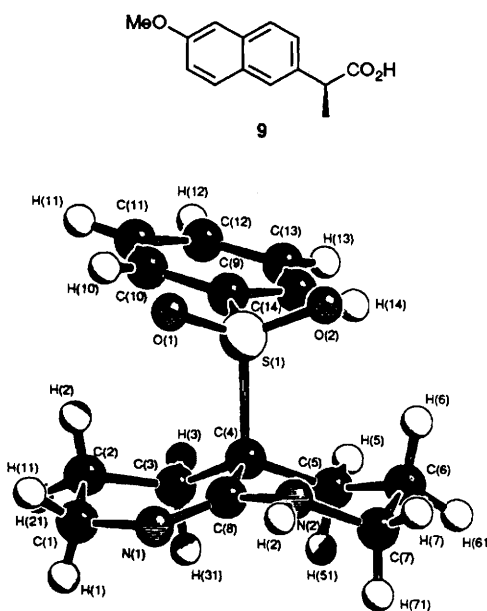
Fig. 1 X-Ray crystal structure of 5
